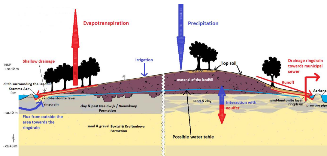
Figuur 5: Geohydrologische doorsnede Coupépolder (bron [lit. 3])
